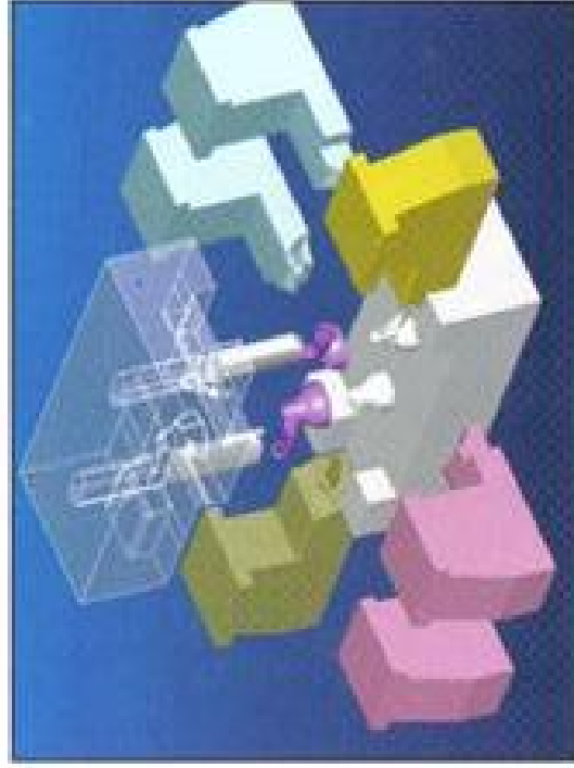
模具結構圖 Mould structure drawing
